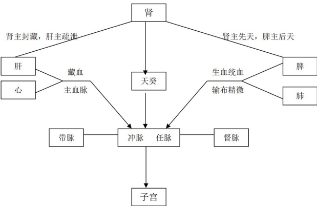
图1 肾-天癸-冲任-子宫轴与其他脏腑、经络的关联示意图 Figure 1 Schematic diagram of the association of the Kidney-Tian gui-Chong ren-Uterus Axis with other viscera and meridians
